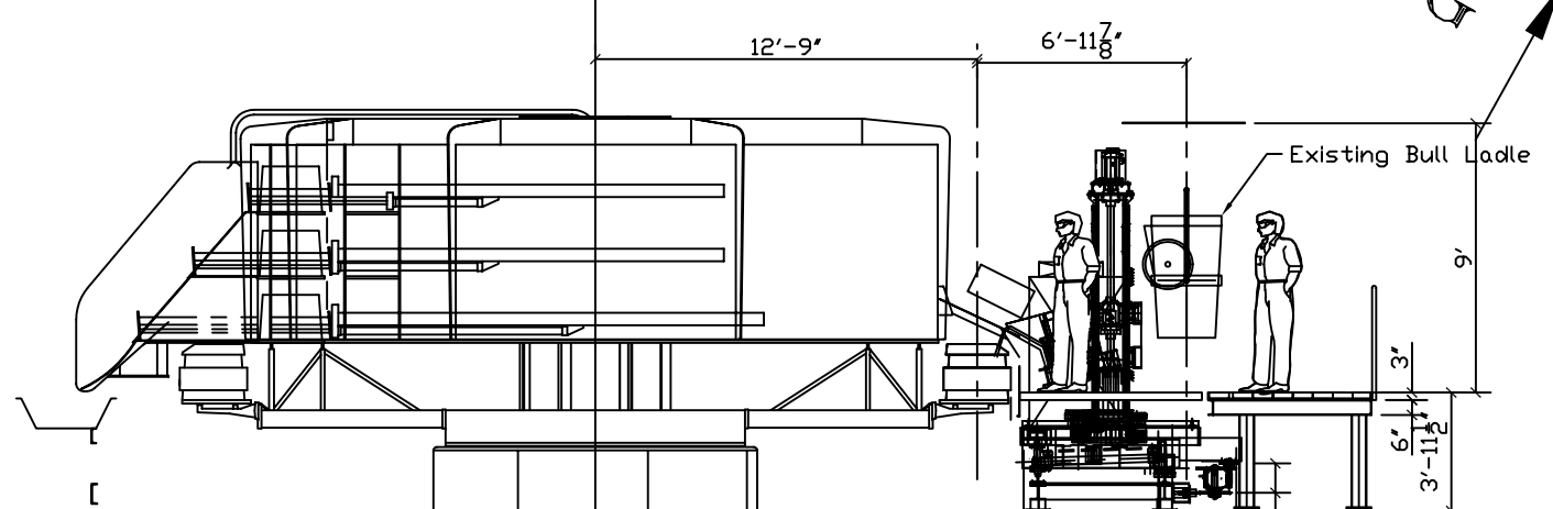
Sectional Elevation G - G
